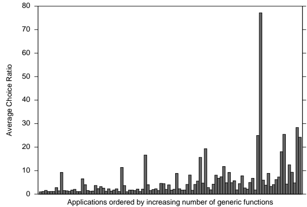
Figure 19. Average choice ratio ( CR_{ave} ) for Java applications.
