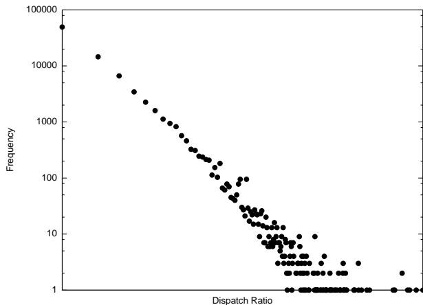
Figure 18. Dispatch ratio (DR) percentage distribution for Java applications, log-log scale.
