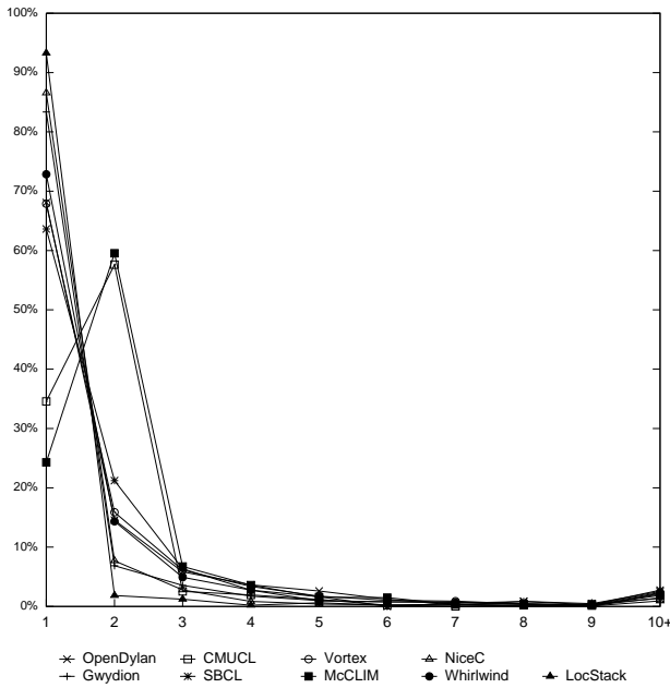
Figure 5. Dispatch ratio (DR) frequency distribution, expressed as a percentage of all generic functions with a given DR measurement.
