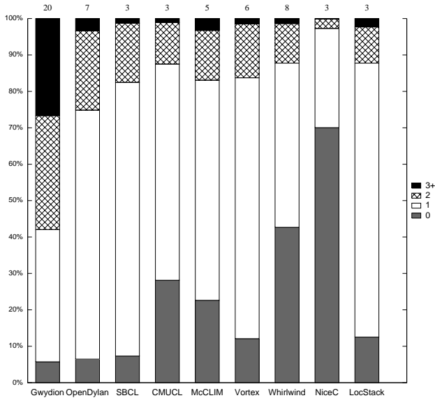
Figure 7. Degree of specialisation (DOS) distribution of concrete methods across applications. The lowest block in each stack is the proportion with DOS measurement of 0, the next, the proportion with 1, and so on. The value at the top of each stack indicates the highest DOS measured for this application.
