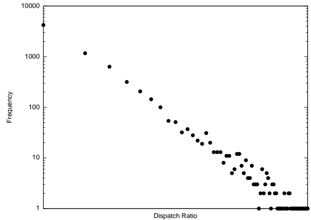
Figure 6. Dispatch ratio (DR) distribution, log-log scale
