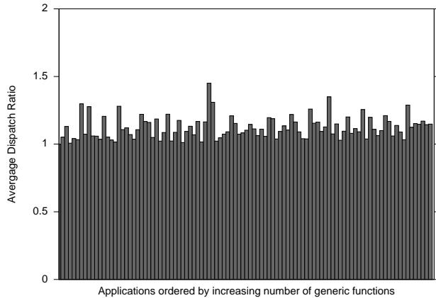
Figure 17. Average dispatch ratio ( DR_{ave} ) for Java applications.
