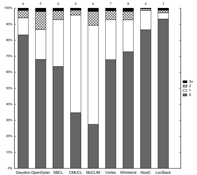
Figure 10. Rightmost dispatch (RD) distribution of generic functions across applications. The value at the top of each stack indicates the highest RD measured for this application.
