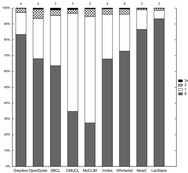
Figure 9. Degree of dispatch (DOD) distribution of generic functions across applications. The value at the top of each stack indicates the highest DOD measured for this application.
